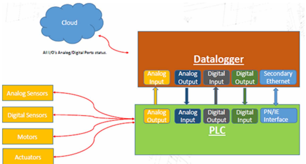
Figure 4. PLC and IIoT input and output lines
