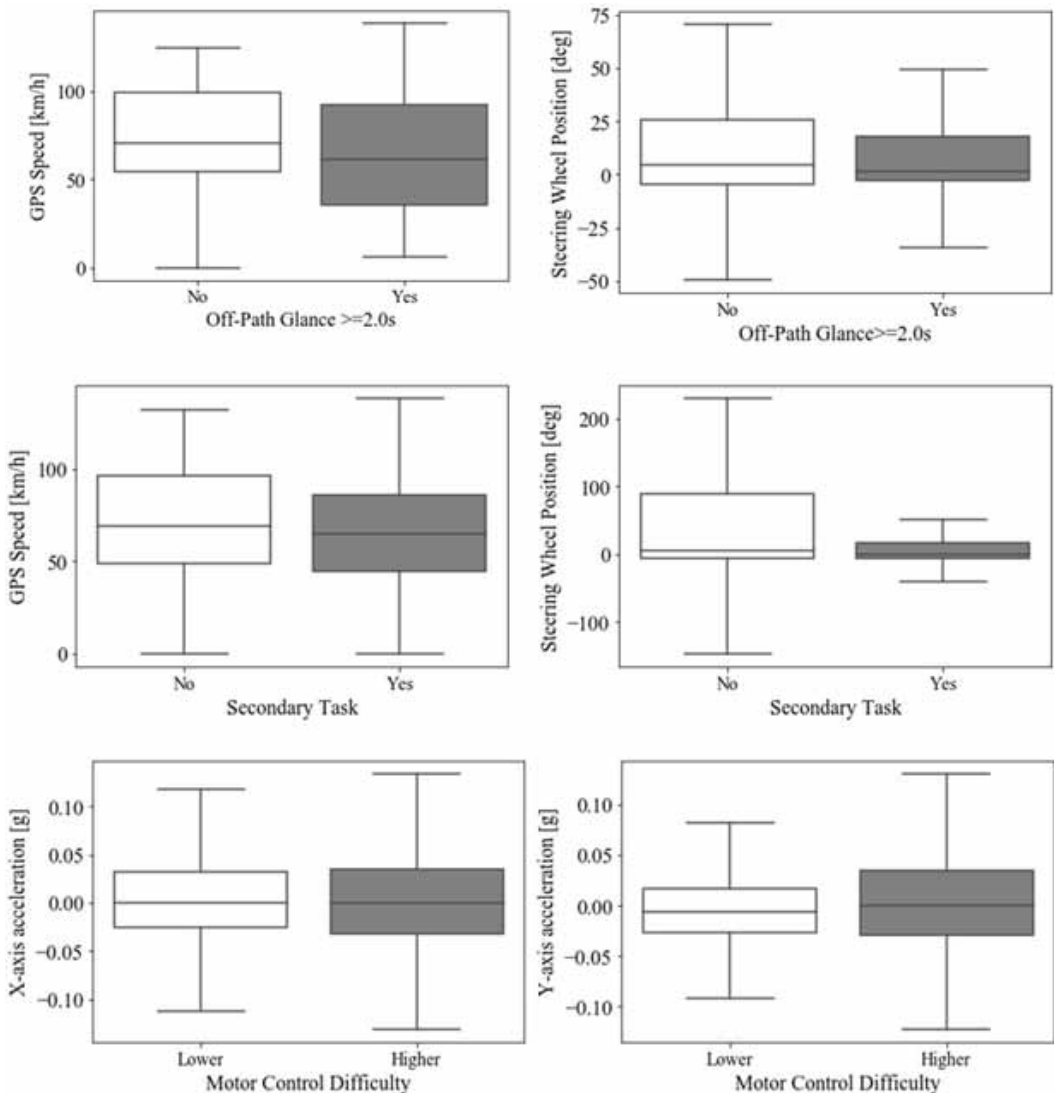
Figure 2. Boxplots of predictor variables across different classes; boxplots depict the five-number summary
