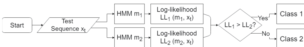
Figure 1. The HMM classification process
