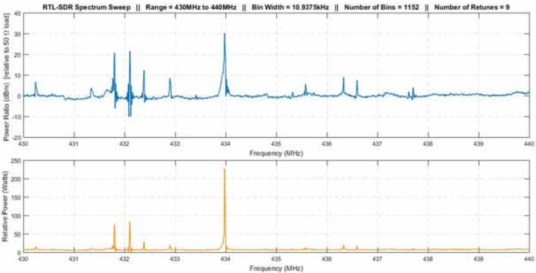
Figure 7. Frequency Sweep around the desired central frequency of 434 MHz detected at Night-Time
