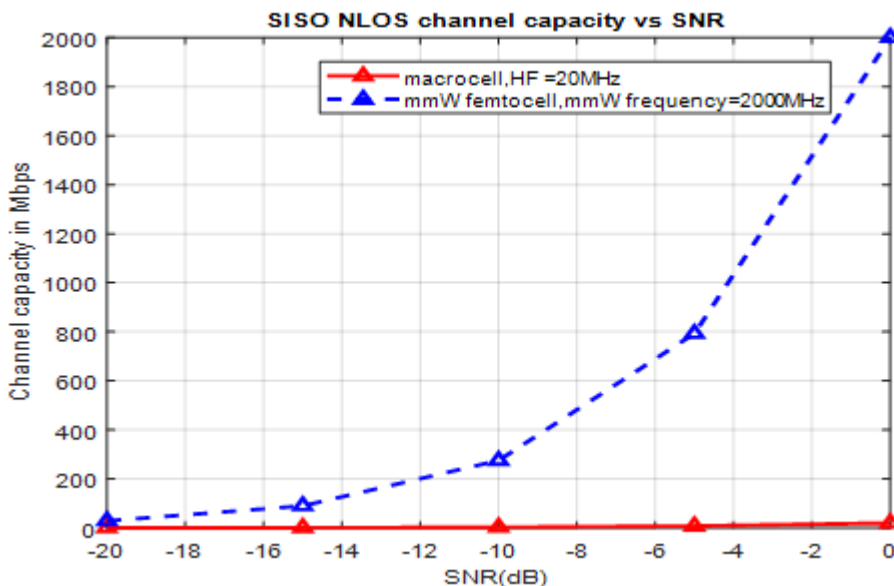
Figure 6a. Effect of SNR variations on the NLOS capacity
