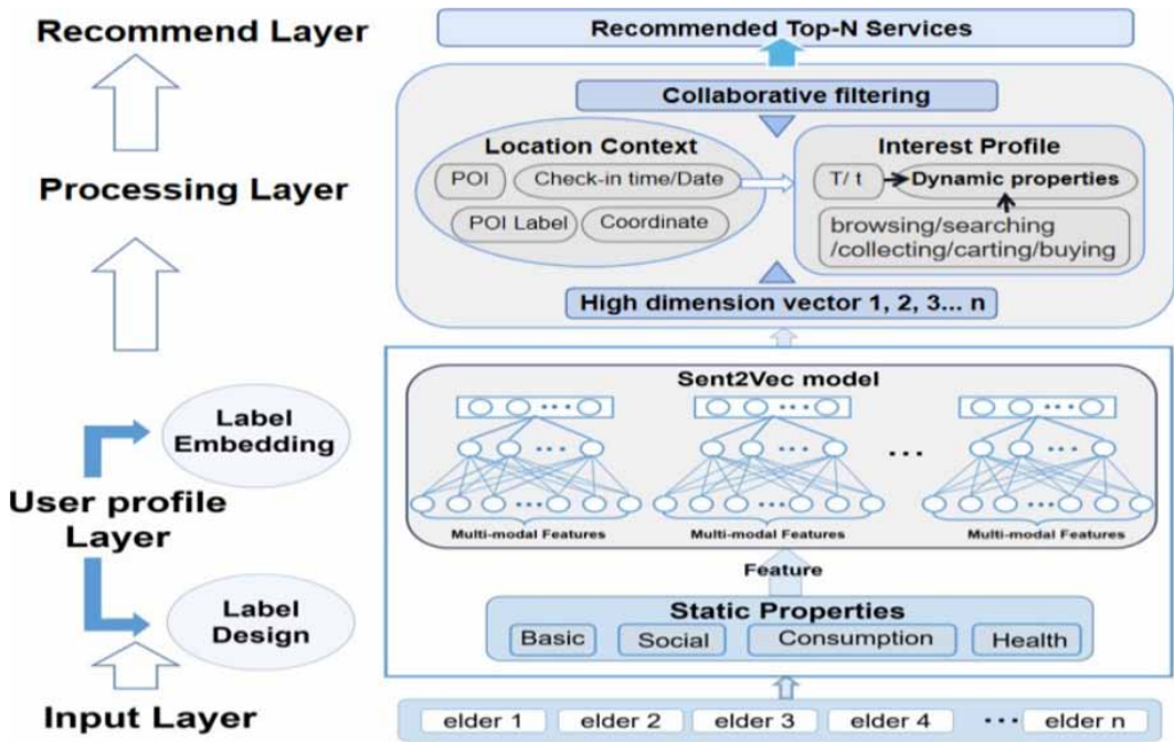
Figure 1. PCE-CF framework
