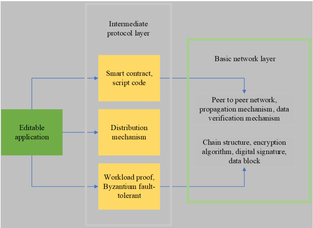
Figure 4. Blockchain infrastructure
