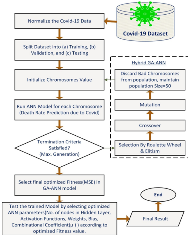
Figure 2. Flowchart of Hybrid GA-ANN Model for Prediction of the death rate due to COVID-19 transmission
