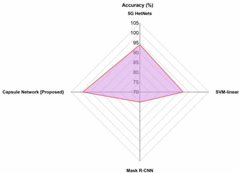
Figure 3. Accuracy comparison
