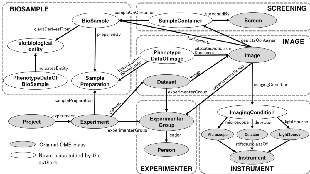
Figure 9. Overview of classes and relations extracted in the RDF-based OME data model and its extension. The circles represent rdfs:Class or owl:Class instances, while the arrows represent their relationships. The grey classes are directly translated from the OME data model and the white classes are the proposed extended classes. The dotted rectangles represent expedient groups of classes for describing the biological sample (biosample) as an object in the image, screening (a type of biological experiment for sorting substances), images, the experimenters who are 'authors' of the image, and the instruments used in imaging experiments. For example, the class ImagingCondition is linked from Image by the relationship, imagingCondition . The 'ome:' prefixes are omitted.
