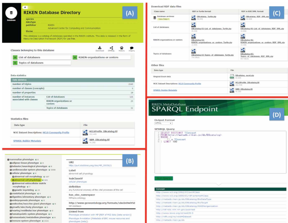
Figure 8. Specialised views: (A) Database view; (B) Ontology tree view; (C) Download view and (D) SPARQL search view
