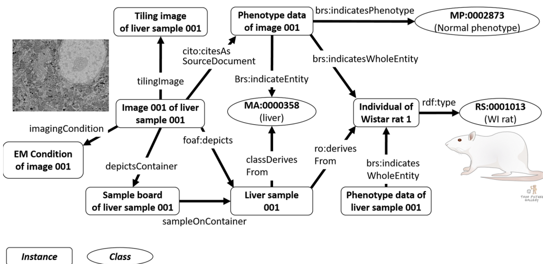
Figure 10. An example of a graph structure that describes imaging data. The rounded rectangles are instances of classes and the ovals are classes. An electron microscope image (Image 001 of liver sample 001) depicts a liver sample (Liver sample 001) derived from a Wistar rat (Individual of Wistar rat 1). Referencing Image 001 of liver sample 001, phenotype data (Phenotype data of image 001) was produced. The graph structure can link the bioresource information in RIKEN to an external database from RS:0001013.
