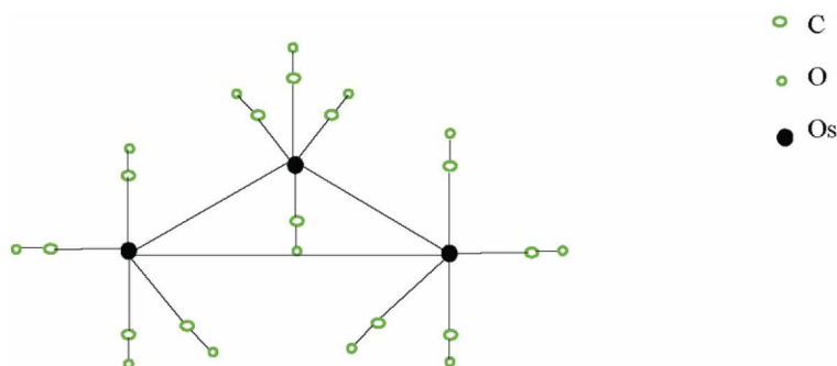
Figure 10. Shema of three - nuclear carbonyls Ru and Os
