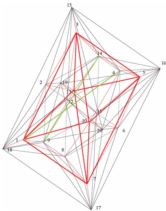
Figure 9. Spatial image of cobalt tetra - anion cluster [Co_6(\mu - Co)_8(CO)_6]^{4-}
