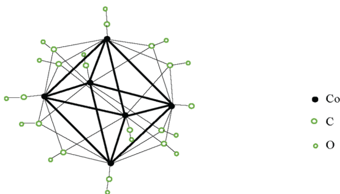
Figure 6. Scheme of cobalt tetra - anion cluster [Co_6(\mu - Co)_8(CO)_6]^{4-}
