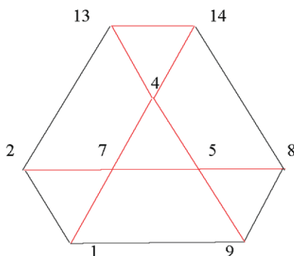
Figure 16. A section dividing a cluster with a three - bar closed cycle of metal atoms into two polytopes
