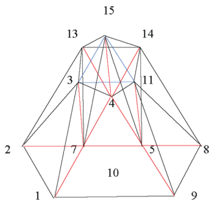
Figure 14. The polytope upper part of a cluster with a three - bar metal atom cycle
