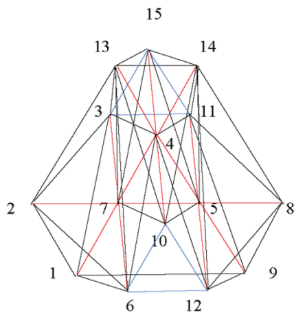
Figure 13. Spatial image of the cluster with a closed three - bar metal cycle
