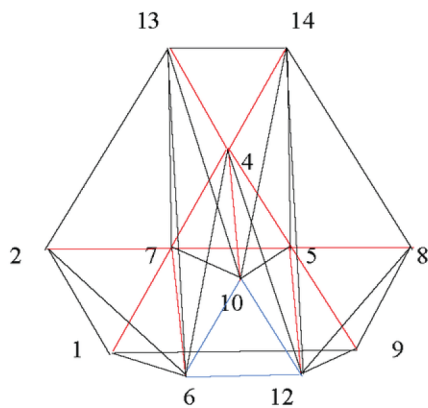
Figure 15. The polytope lower part of a cluster with a three - bar metal atom cycle
