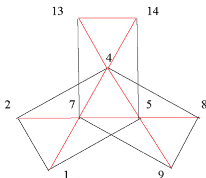
Figure 12. A section of a cluster containing a closed three - bar metal cycle
