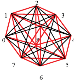
Figure 1. The octahedron with attached tetrahedrons on faces of octahedron
