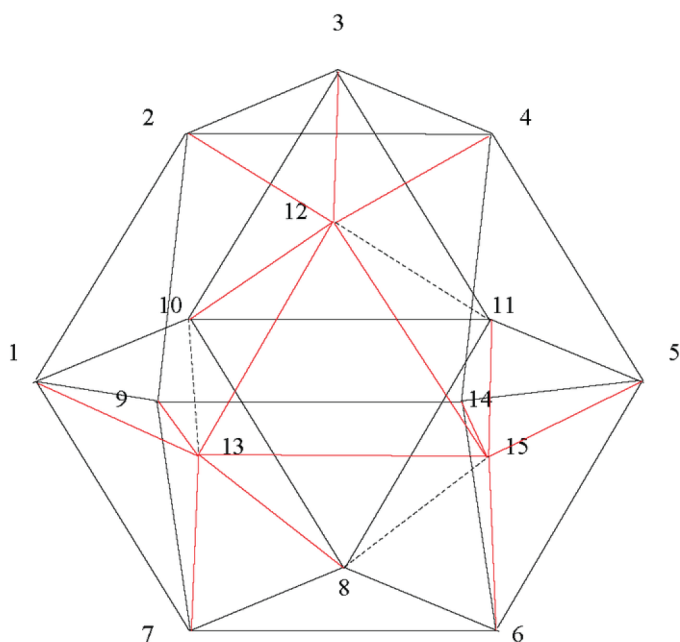
Figure 11. The anti - cube - octahedron with the three nuclear metal cycle
