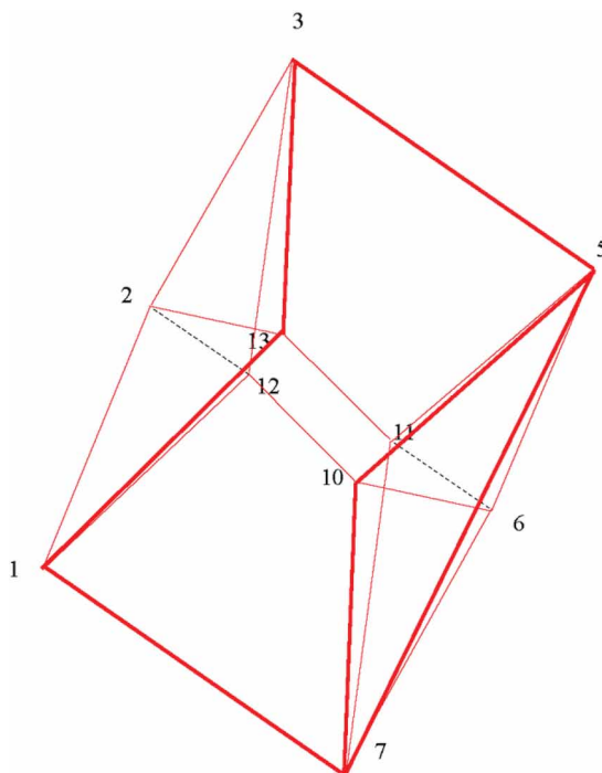
Figure 8. The image a closed body S = 2 - 13 - 11 - 10 - 6 - 12 - 3 - 5 - 1 - 7
