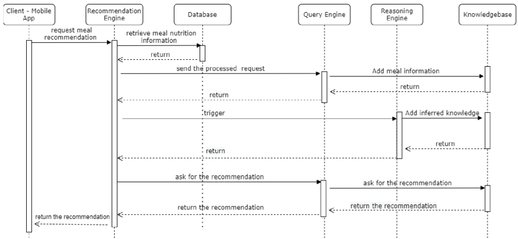
Figure 4. Sequence Diagram of the Recommendation Request.
