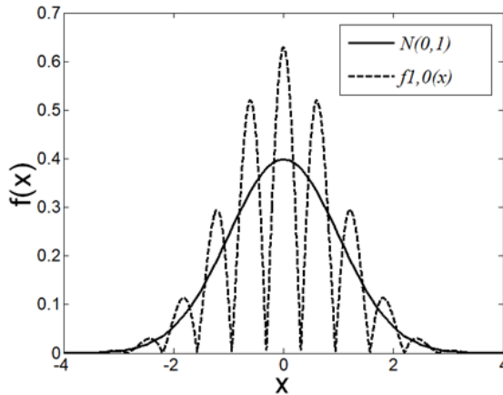
Figure 1. Image of f_{1,0}(x) and N(0,1)
