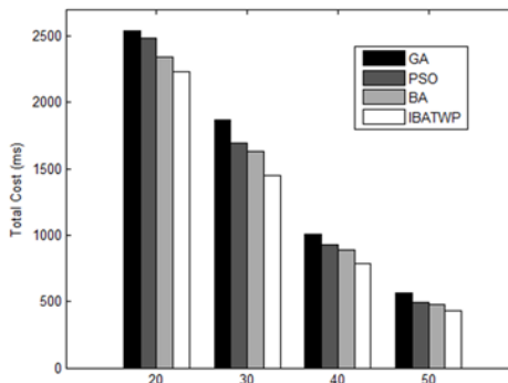
Figure 8. The Impact of the Number of Virtual Machines on Total Cost
