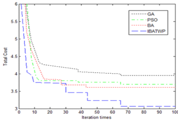
Figure 4. Comparison on Consumption
