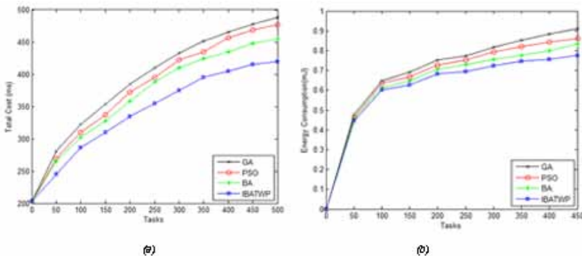
Figure 4. Comparison on Consumption
