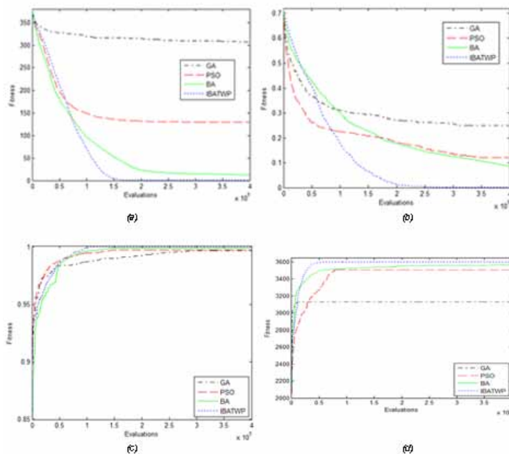
Figure 2. Convergence Curves of f_1 \sim f_4 in Picture (a) ~ (d), respectively
