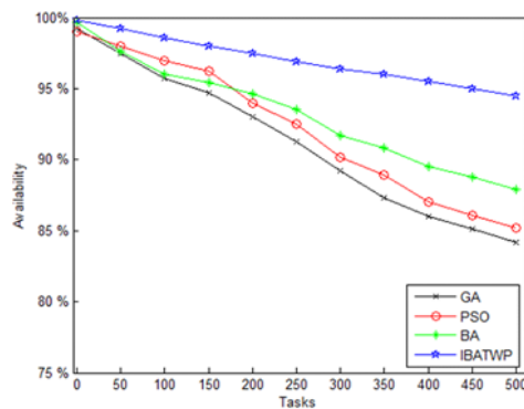
Figure 5. Comparison Availability of Three Resource Scheduling Algorithms
