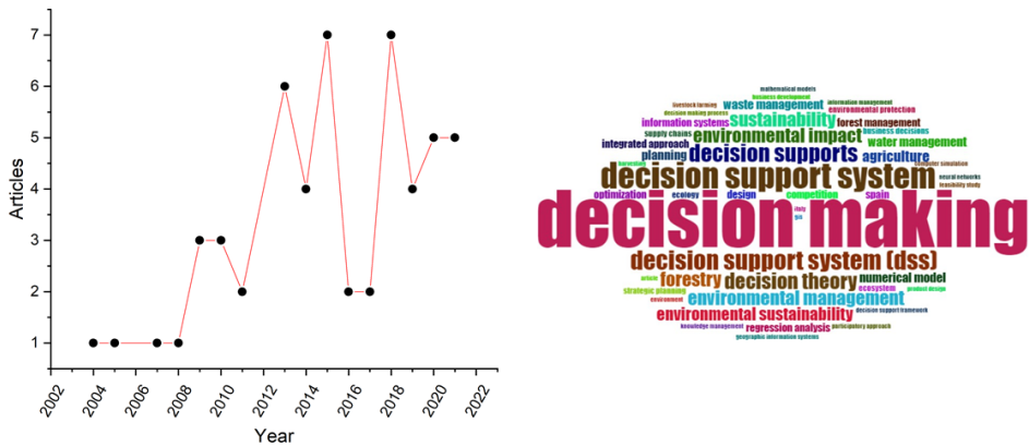
Figure 2. Statistical Results
