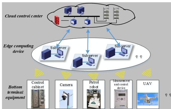
Figure 1. Cloud edge collaborative structure of smart substation
