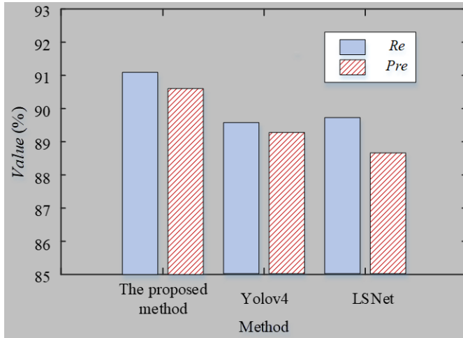
Figure 11. Insulator status identification
