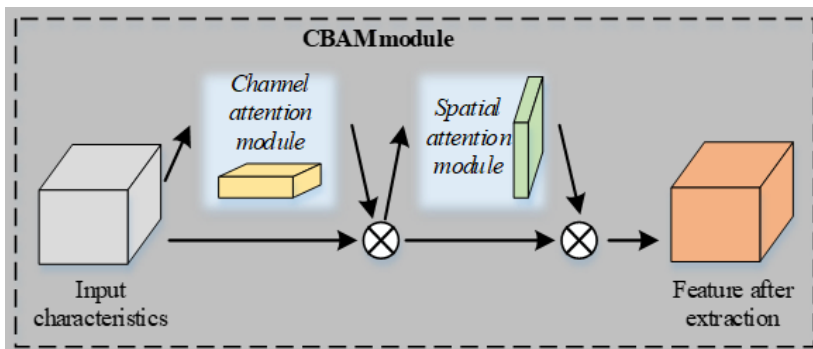
Figure 7. Model structure block diagram of CBAM
