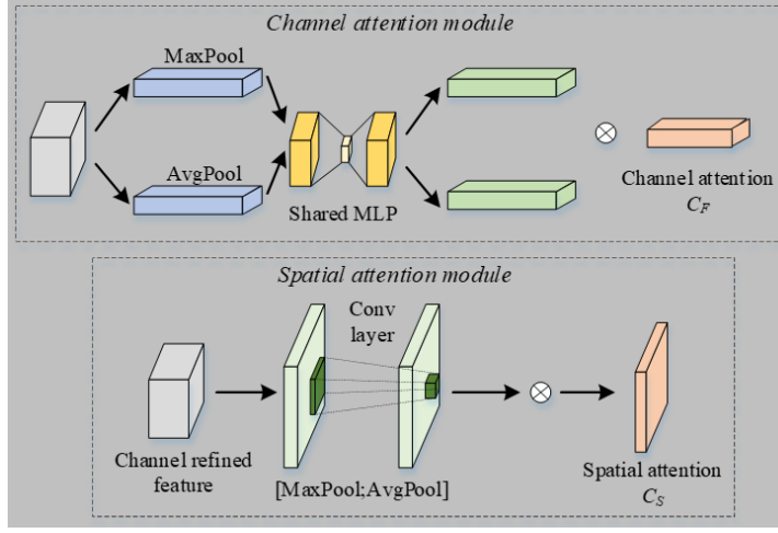
Figure 8. Attention sub-module
