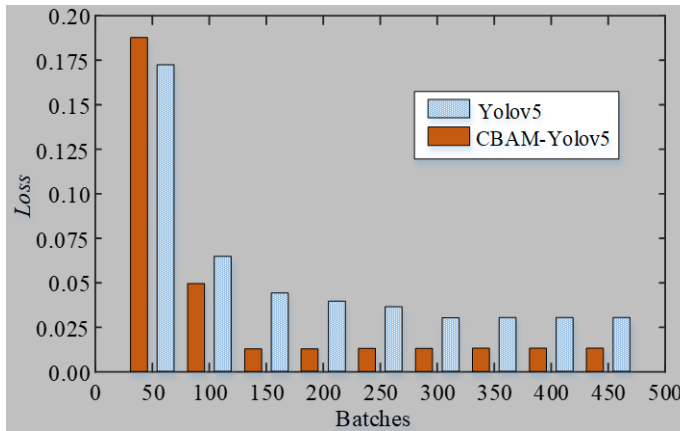
Figure 10. Loss comparison between CBAM-Yolov5 and Yolov5
