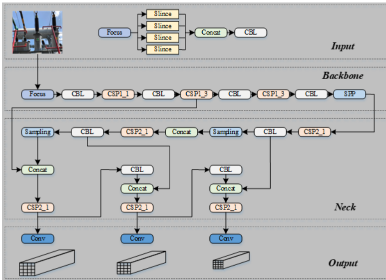
Figure 4. Structure chart of YOLOv5
