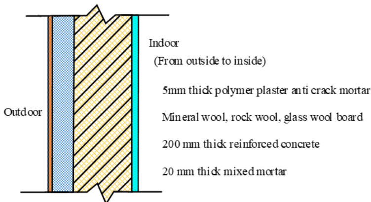
Figure 2. Construction composition of the exterior wall in cold areas
