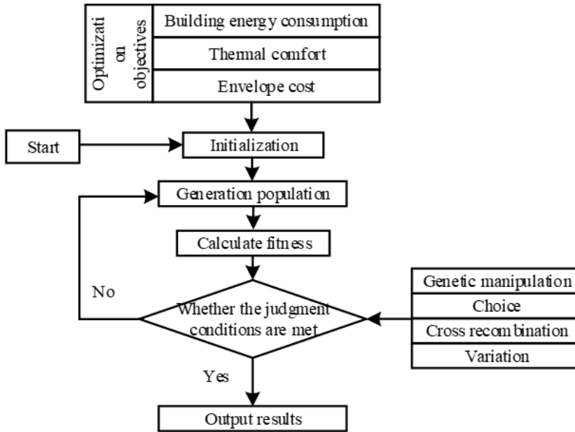
Figure 1. Flow chart of the building energy saving optimization model
