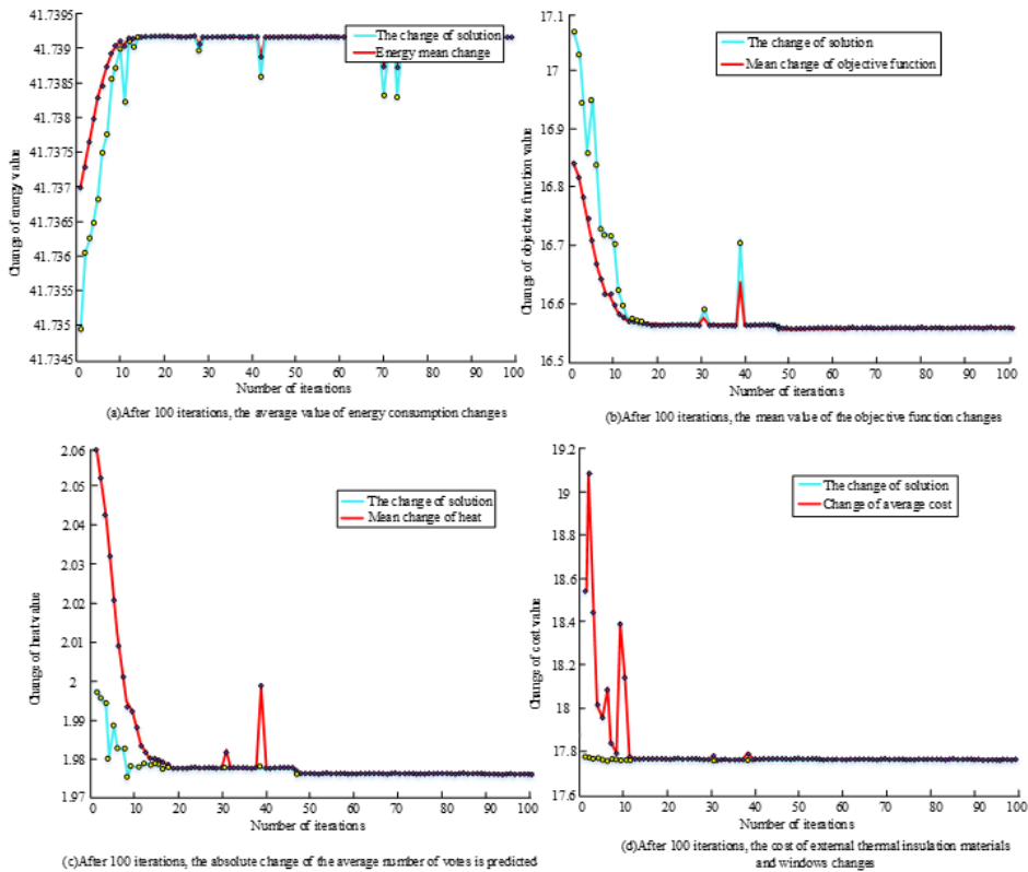
Figure 5. The change of each index after 100 iterations in hot summer and warm winter regions
