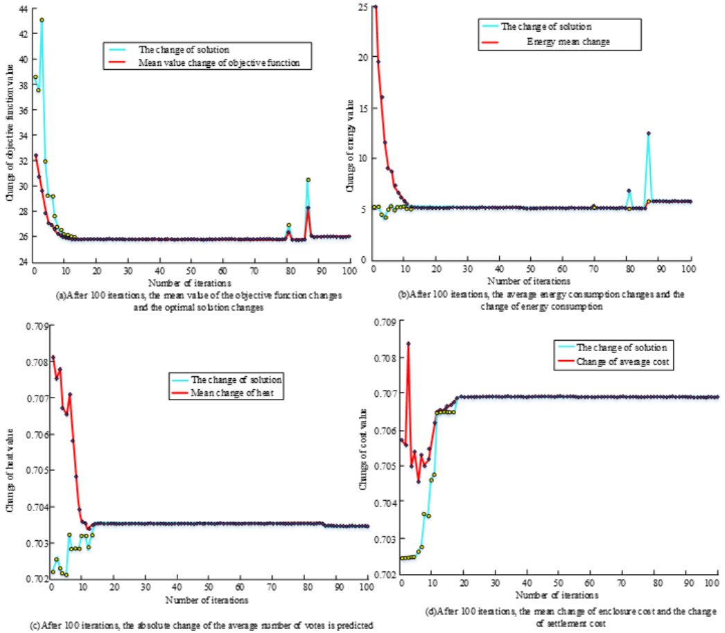
Figure 4. Changes in the enclosure cost, PMV, building energy consumption, objective function, and optimal solution in cold areas
