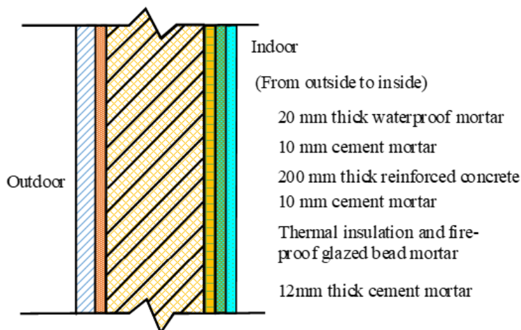
Figure 3. Construction composition of exterior walls in hot summer and warm winter areas
