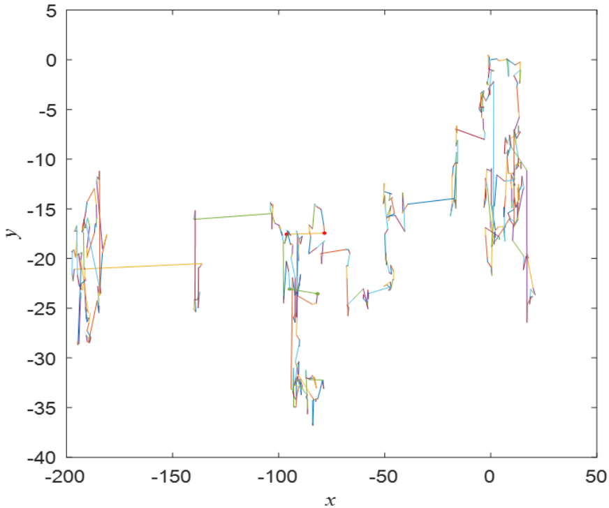
Figure 1. A Lévy flight diagram with 500 steps
