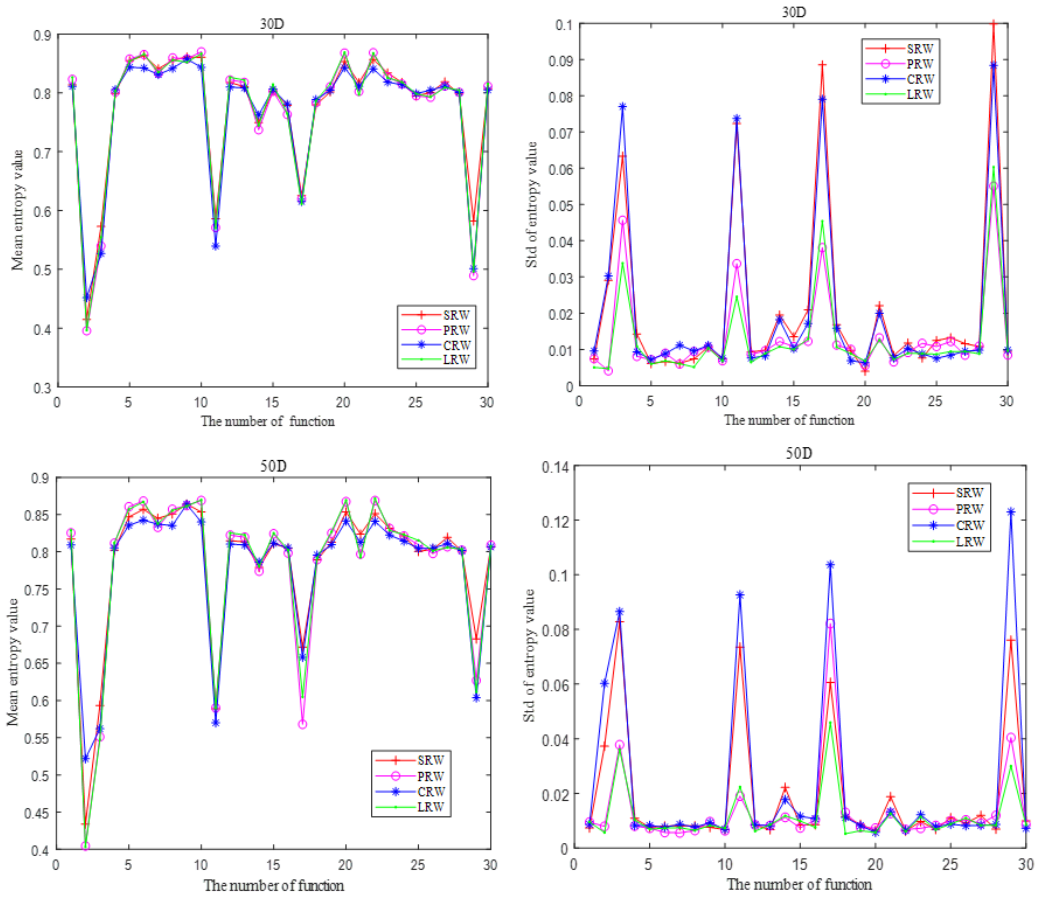
Figure 8. Mean and standard deviation of entropy value for all random walk algorithms with different dimensions
