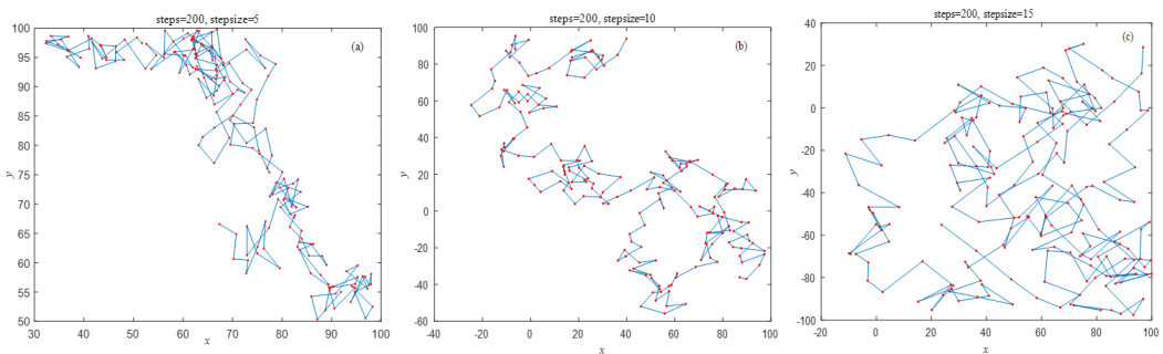
Figure 3. One independent sample walk of 200 steps with variable step size by PRW; (a) s = 5 , (b) s = 10 , (c) s = 15
