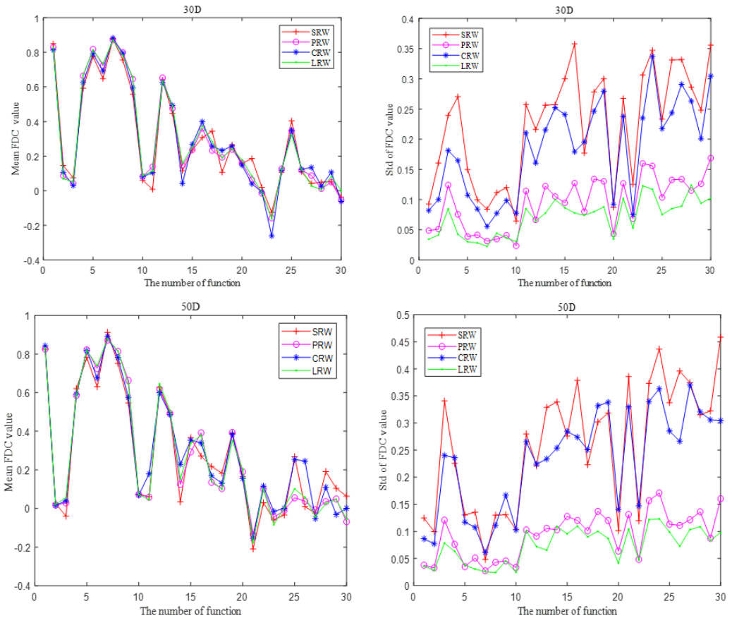
Figure 7. Mean and standard deviation of FDC value for all random walk algorithms with different dimensions
