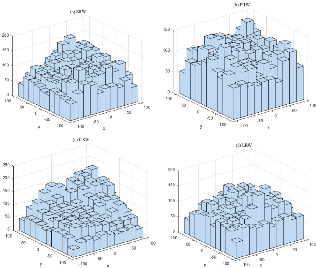
Figure 6. Histogram of four random walk algorithms for a sample of 10000 points
