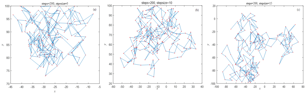
Figure 4. One independent sample walk of 200 steps with variable step size by CRW; (a) s = 5 , (b) s = 10 , (c) s = 15
