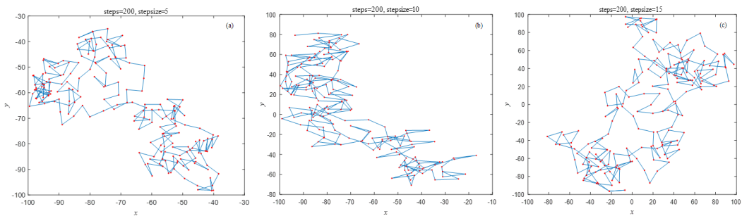
Figure 2. One independent sample walk of 200 steps with variable step size by SRW; (a) s = 5 , (b) s = 10 , (c) s = 15
