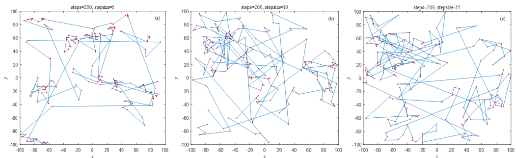
Figure 5. One independent sample walk of 200 steps with variable step size by LRW; (a) s = 5 , (b) s = 10 , (c) s = 15
