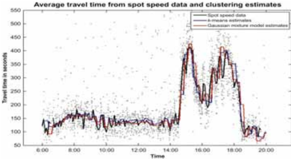
Figure 7. Travel time estimates of the clustering algorithms over the spotted area
