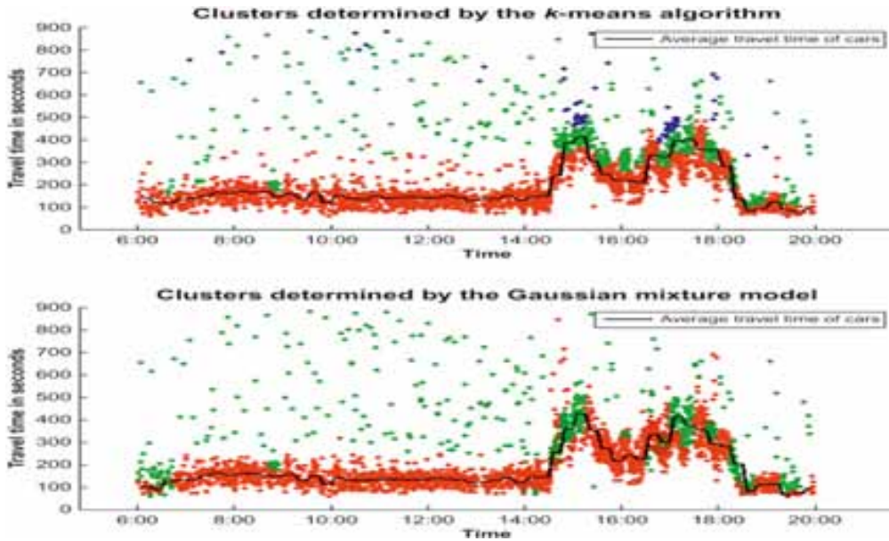
Figure 5. Clusters of traffic density estimates for week
