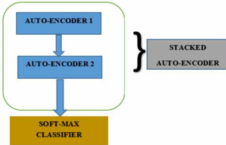
Figure 6. Process of stacked auto-encoder with soft-max classifier
