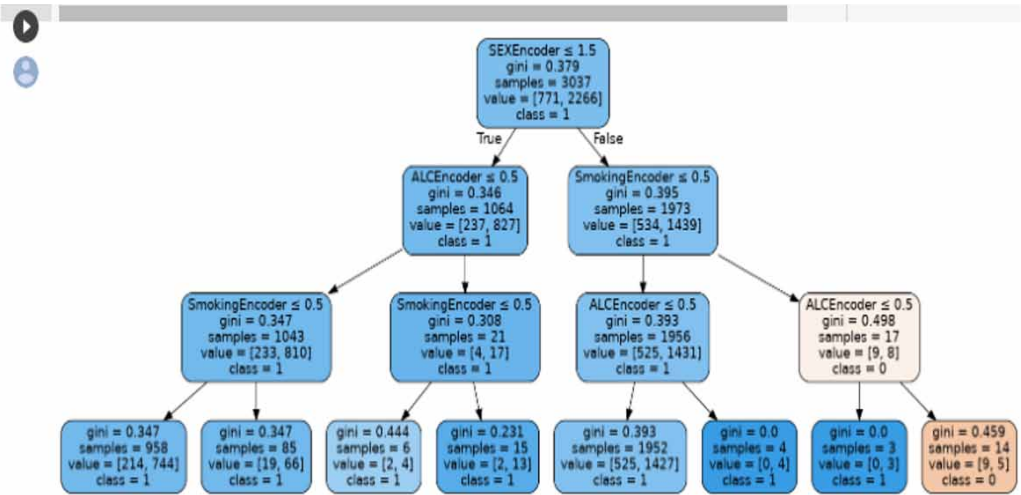
Figure 14. Decision tree classification algorithm using Python based on CKD
