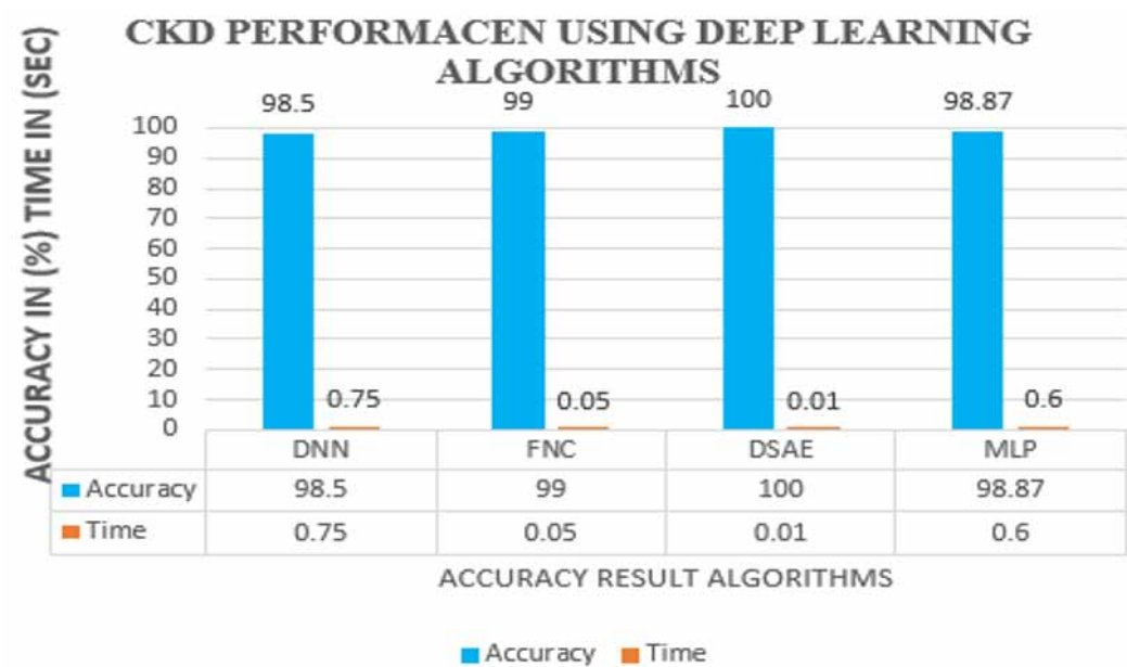
Figure 16. Accuracy performance using various deep learning algorithms
