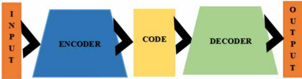
Figure 5. Auto-encoder architecture
