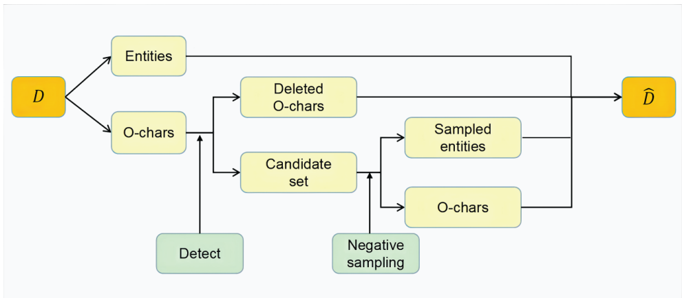
Figure 4. The architecture of our two-step method, in which the pu-learning and negative-sampling approaches are encountered (Note: D is the original dataset and \hat{D} is the modified dataset)
