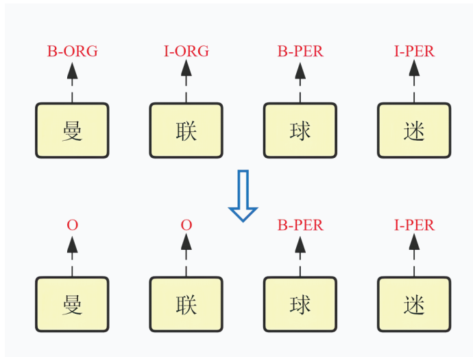
Figure 1. Unlabeled-Entity problem
