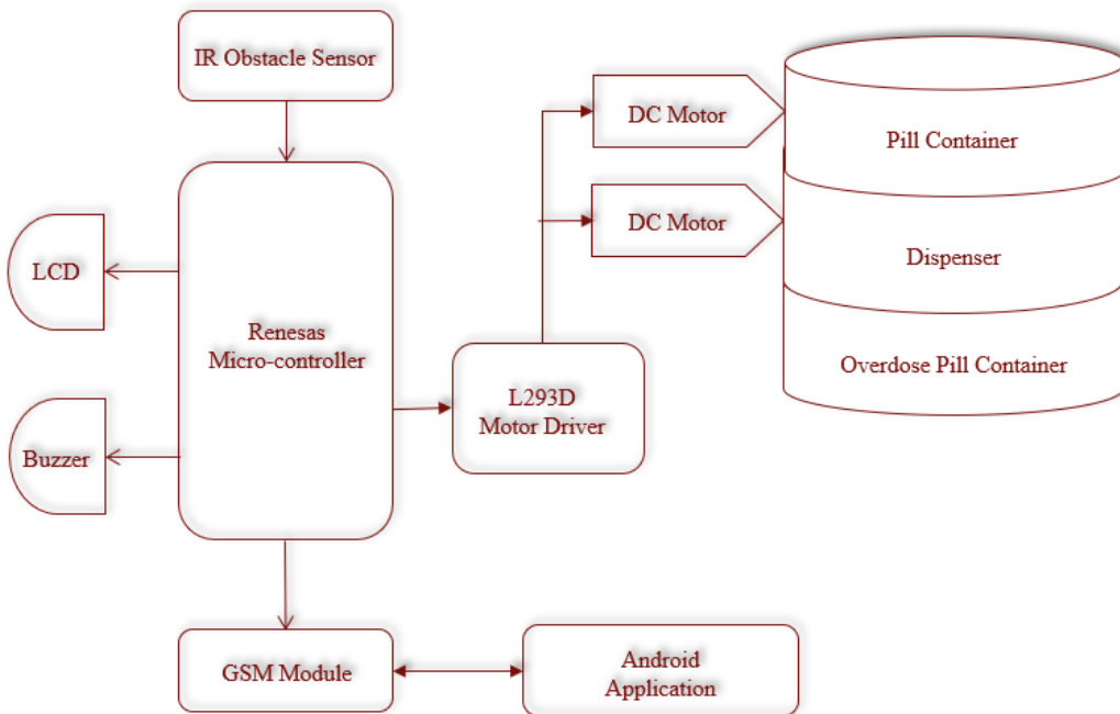
Figure 3. Block diagram of SPEC 2.0
