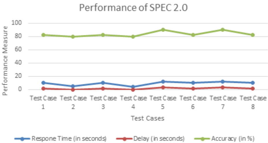
Figure 10. Accuracy and performance graph of SPEC 2.0
