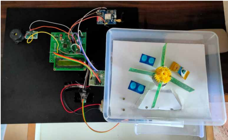
Figure 6. SPEC 2.0 top view
