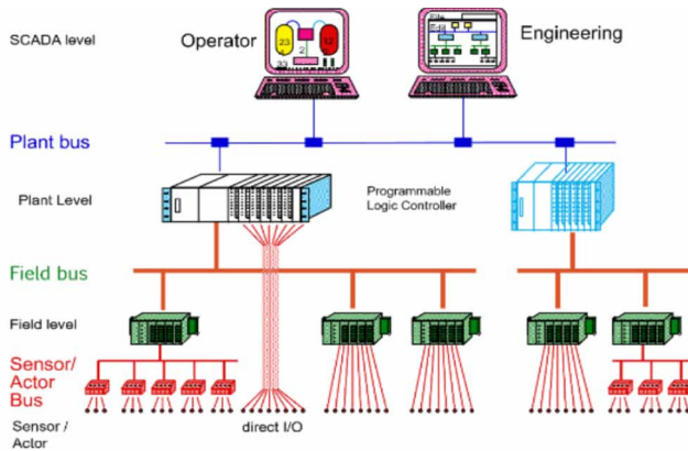
Figure 2. Hierarchical Model of Industrial Networks
