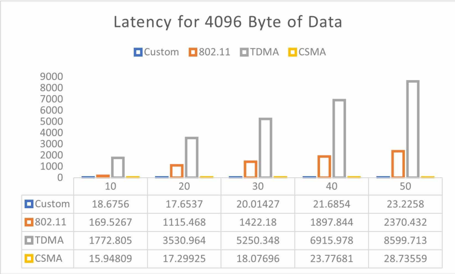
Figure 23. Latency for 4096 Bytes of Data
