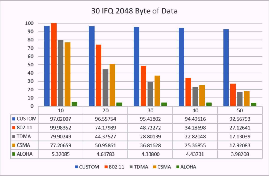
Figure 12. PDR for Packet Size = 2048 Bytes
