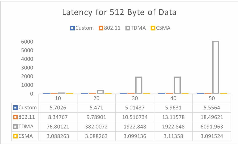
Figure 20. Latency for 512 Bytes of Data
